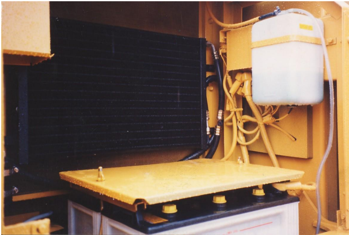
Right side of condenser with bolts in place through flange.
