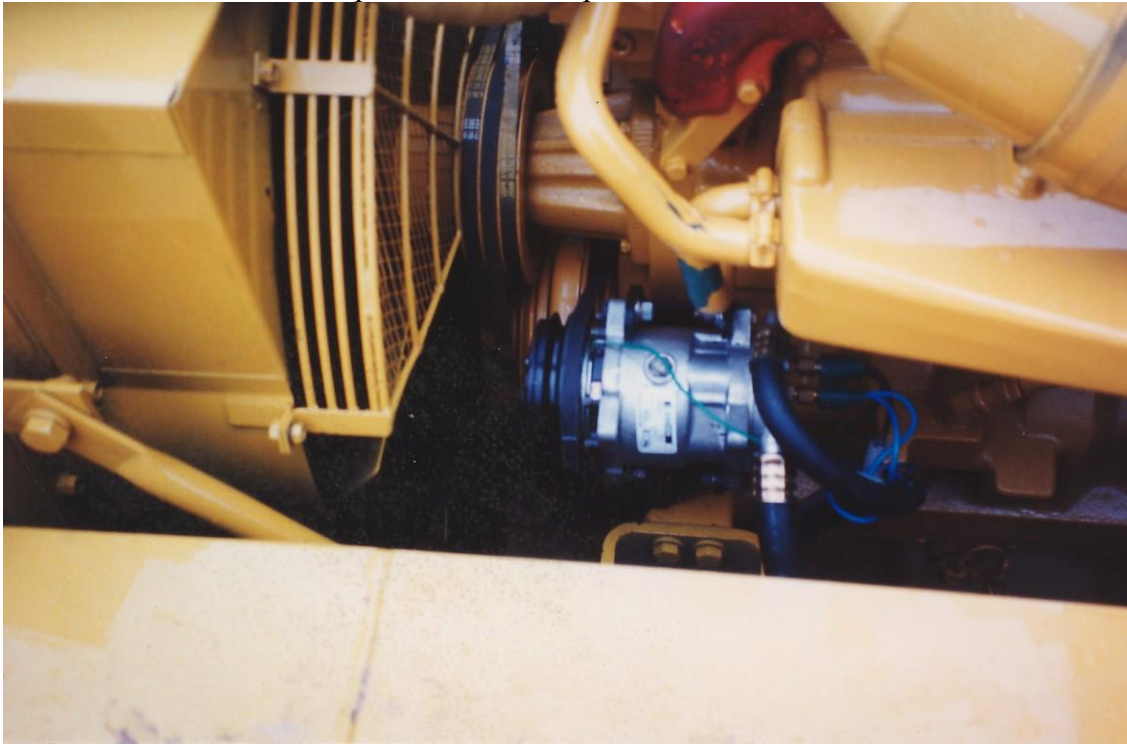
Compressor and mount in place on engine. View from top side of engine compartment.
